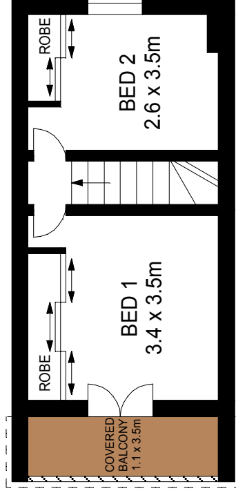
GROUND LEVEL
