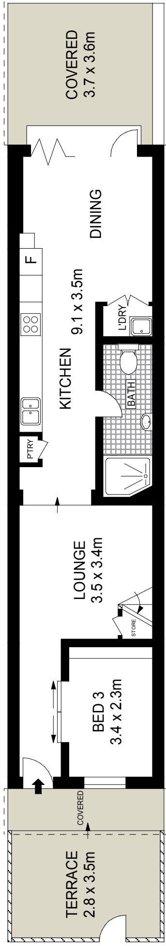
GROUND LEVEL
