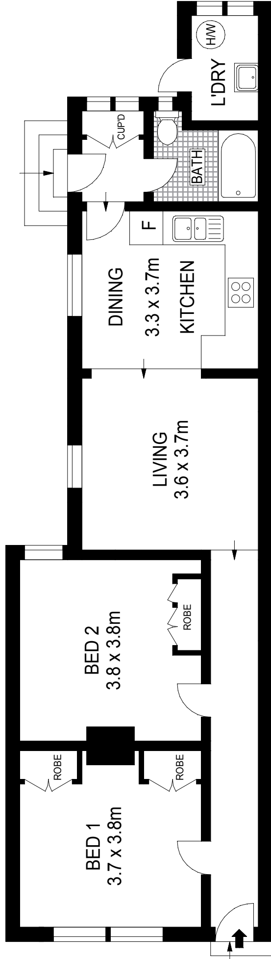
GROUND FLOOR
