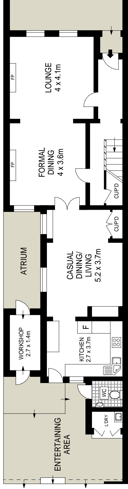
GROUND FLOOR
